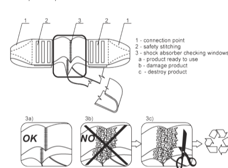
Fig.6 Inspection points
